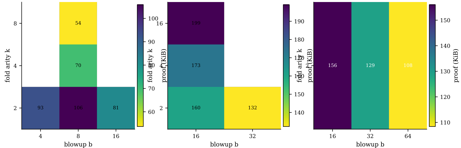
Figure 3. Per-AIR (k, b) STIR proof-size surface at L1/sha3-256/q=2 40 — optimum inverts between AIR scales
