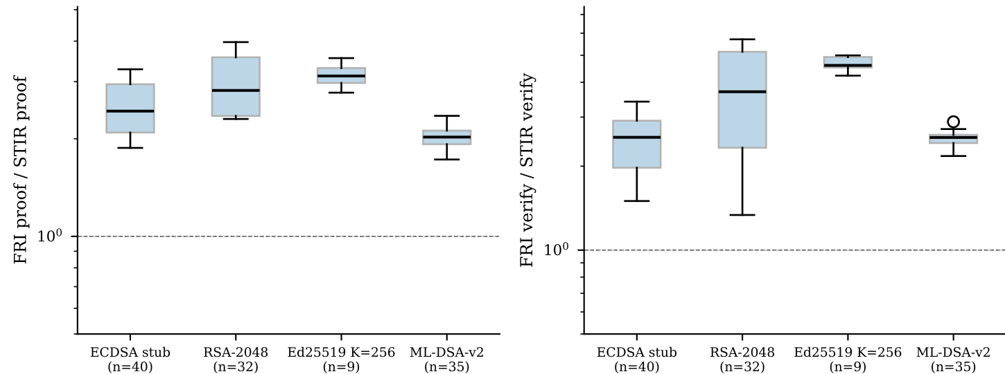
Figure 5. STIR's proof-size and verify-time wins across all matched cells ( >1 = STIR wins)
