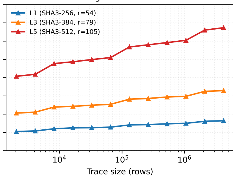
RegisterMachine
