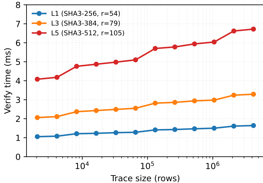
Fibonacci
