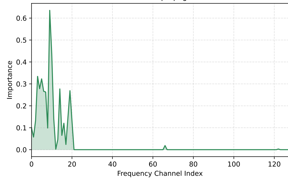
Guided Backpropagation
