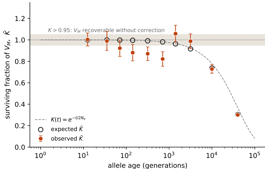
B Kernel is flat across the young bins
