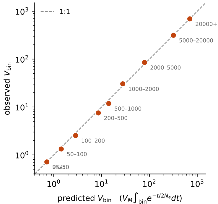
A Per-bin variance matches the neutral kernel
