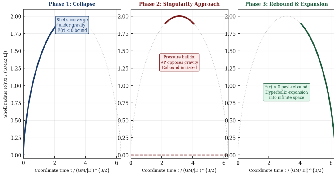
Figure 2. LTB shell dynamics during collapse-rebound. Inner shells reach nuclear density first and rebound outward while outer shells are still infalling, creating the kinematically complex early-universe environment responsible for BBN and CMB.
