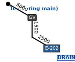
Detail C: CW-205 DN100 (not to scale)
