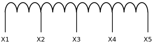
secondary winding (multi-ratio)
