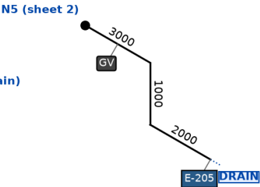
Detail F: CW-209 DN80 (not to scale)
