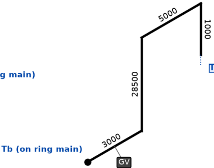
Detail B: CW-204 DN150 (not to scale)
