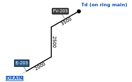
Detail D: CW-206 DN100 (not to scale)
