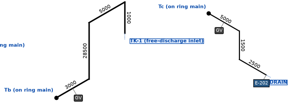
Detail C: CW-205 DN100 (not to scale)
