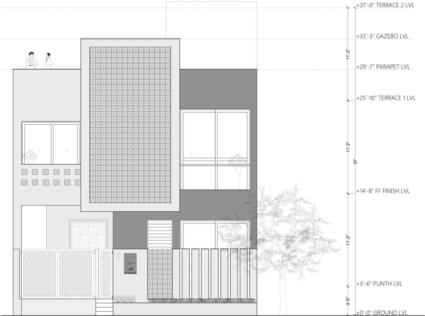
Front Elevation
