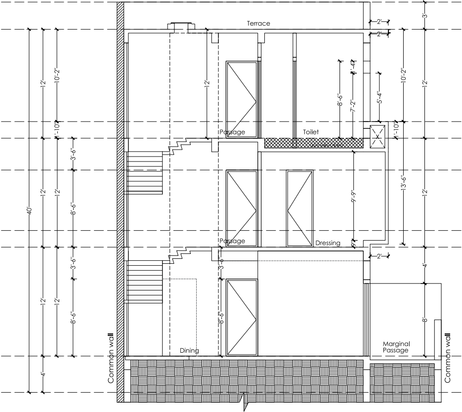
Section C-C'
