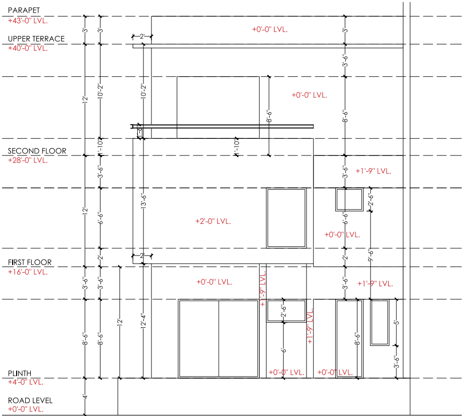
Rear Elevation
