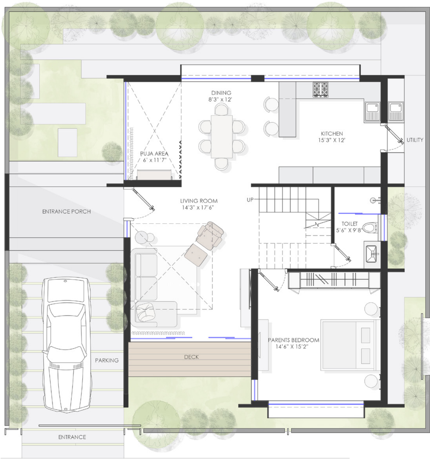
Ground Floor
