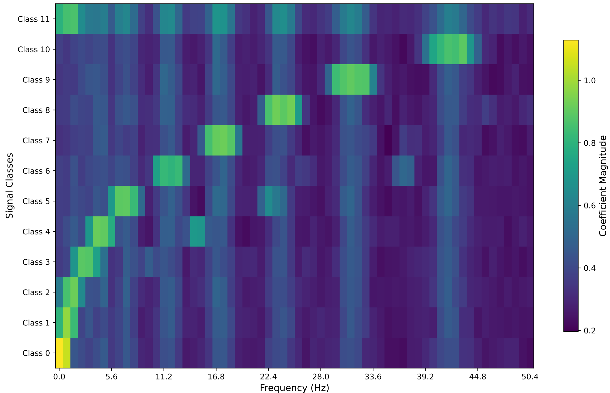
Frequency Importance Heatmap (Biosignal Classification - STFT-KAN)
