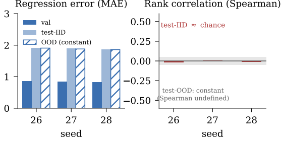
Figure 1: The value-head diagnostics: the rank and OOD probes expose what error metrics alone would miss. Targets are remaining witness steps, bounded above by four. Left: regression error (validation MAE 0.847/0.838/0.830, test-IID MAE 1.92/1.89/1.87 across seeds 26/27/28); the hatched bar is the model’s own constant OOD predictor at MAE 1.91/1.88/1.86—indistinguishable from the trained test-IID error. Right: the same model ranks at chance (test-IID Spearman -0.014/0.002/-0.009 , \approx 0 , grey band), and the constant OOD predictor’s Spearman is undefined. Error alone would pass it; the rank and OOD probes fail it.
