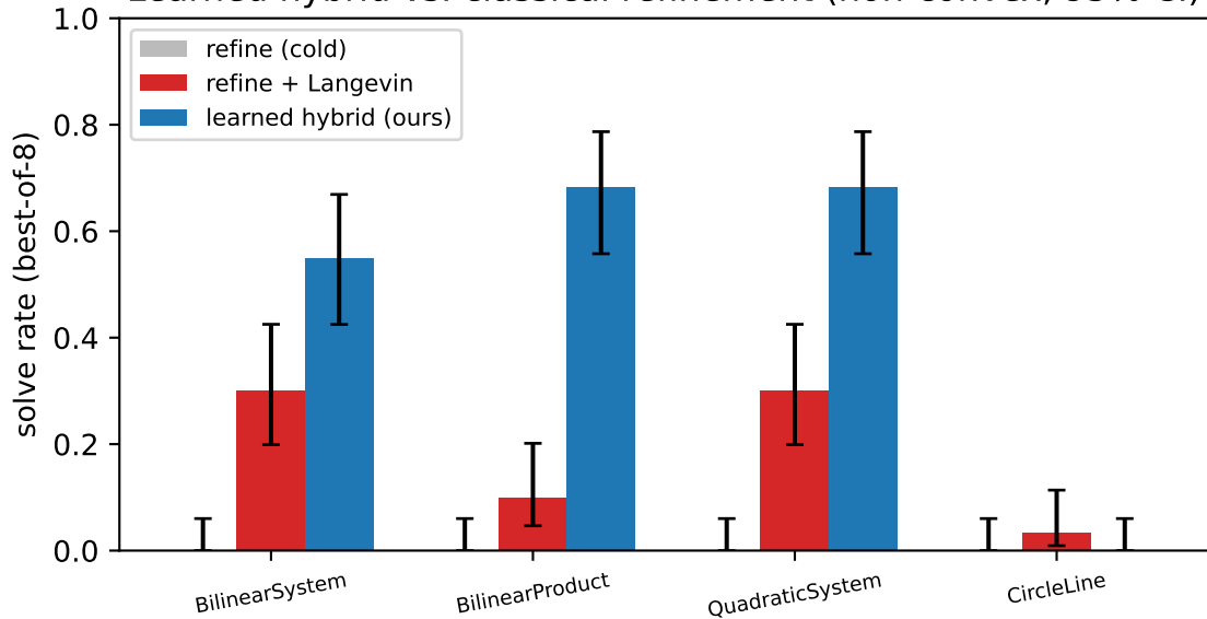
Learned hybrid vs. classical refinement (non-convex, 95% CI)
