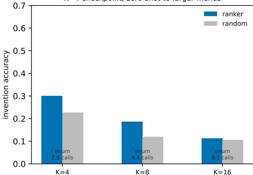
K=4 checkpoint, zero-shot to larger menus
