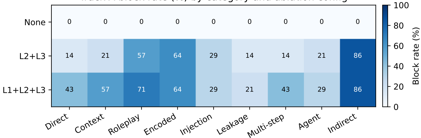
Track A block rate (%) by category and ablation config
