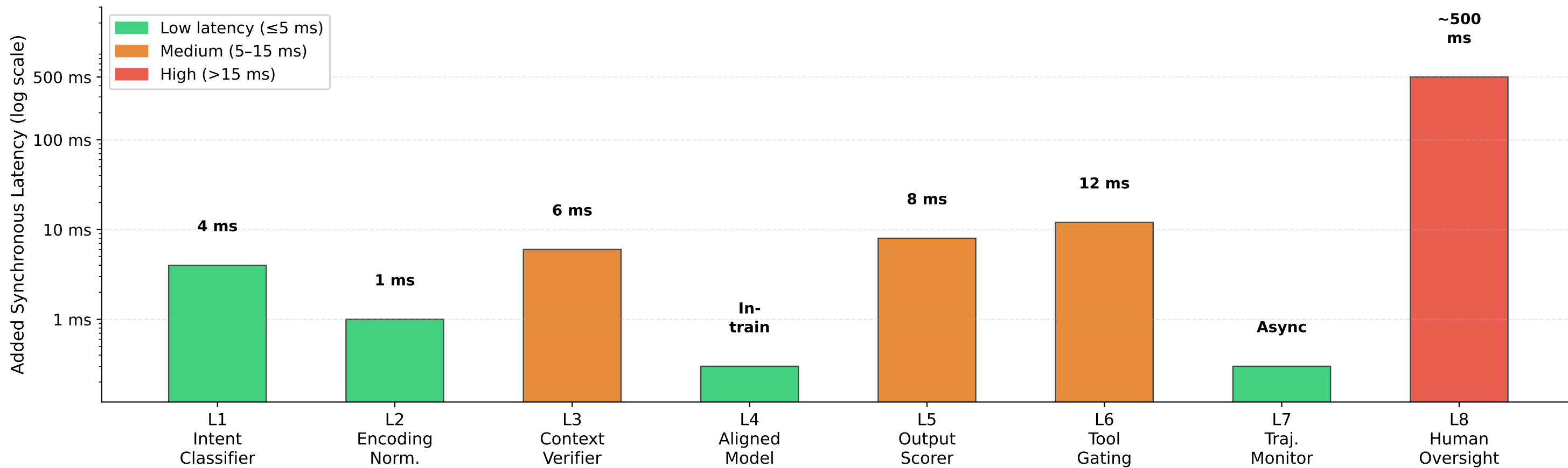
Per-Layer Added Synchronous Latency Green \leq 5 ms · Orange 5-15 ms · Red > 15 ms · 'In-train' / 'Async' = zero sync cost
