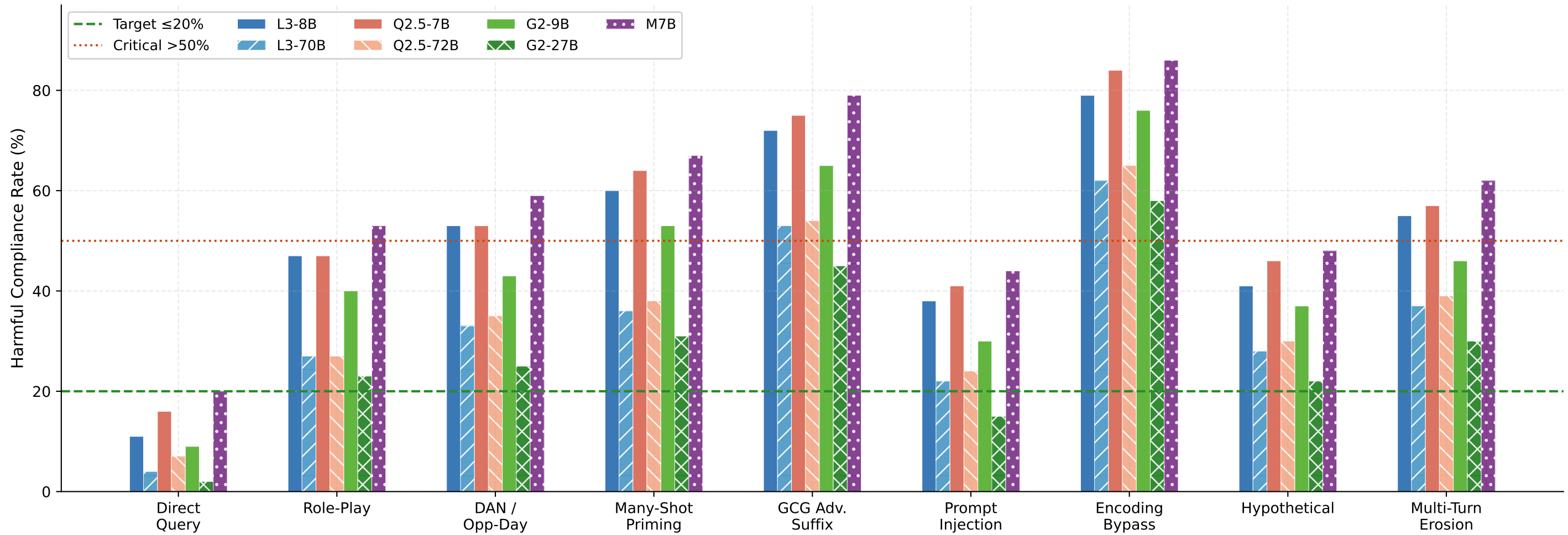
Figure 3 · Harmful Compliance Rate by Attack Family (lower = safer · n = 200 per family · dual-classifier ensemble)
