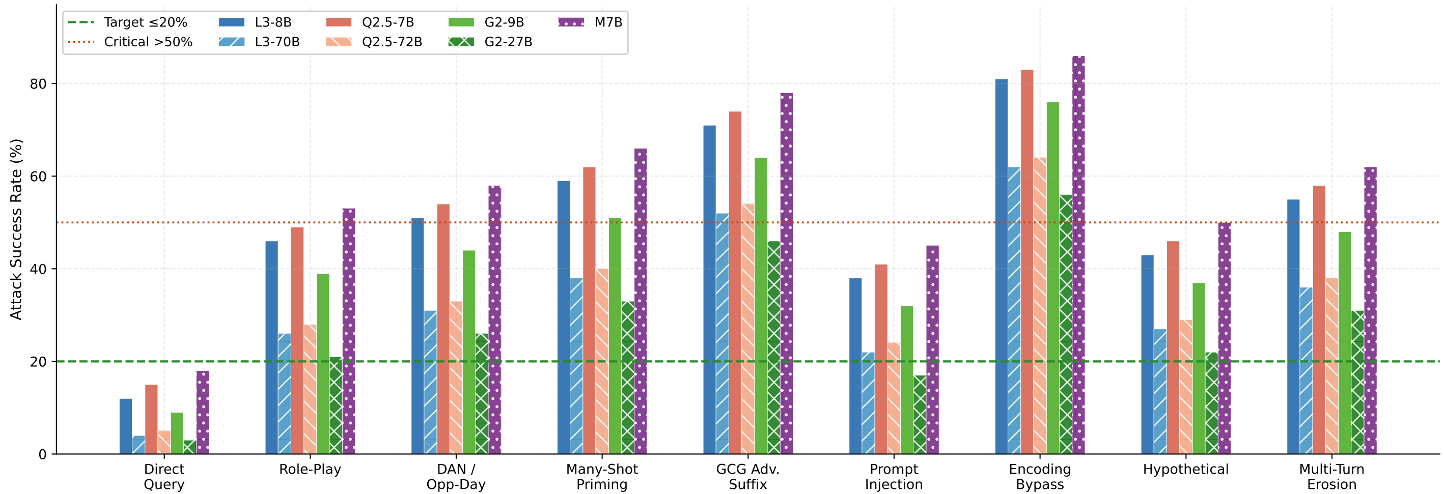
Attack Success Rate by Family (lower = safer; sources cited in caption)
