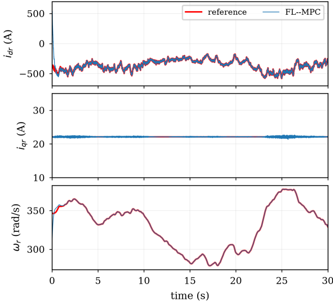
Fig. 5. Tracking performance of the state variables i_{dr} , i_{qr} , and \omega_r under the proposed hybrid control scheme.
