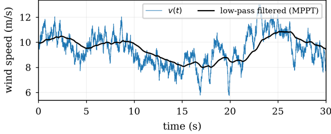
Fig. 2. Wind-speed trajectory.
