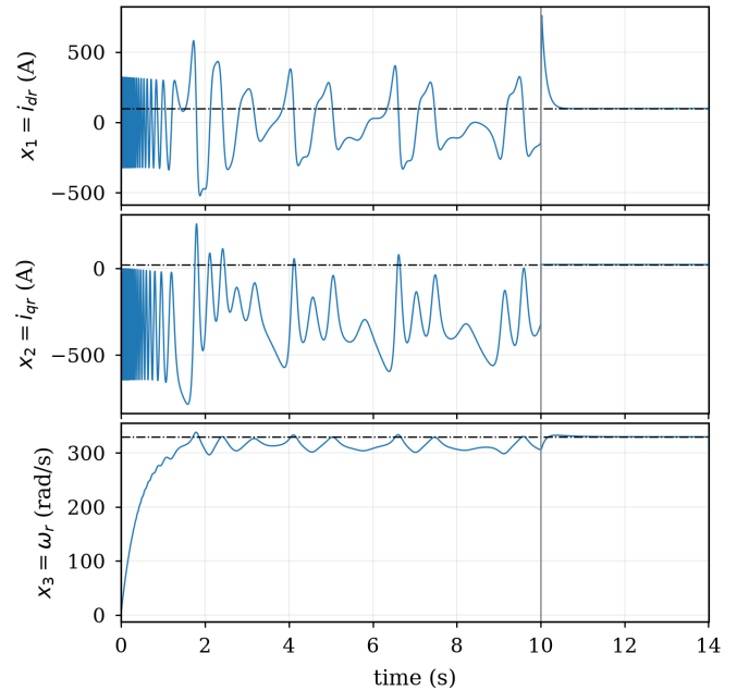
Fig. 4. Time evolution of the state variables before and after control activation at t = 10 s (dash-dot: target).
