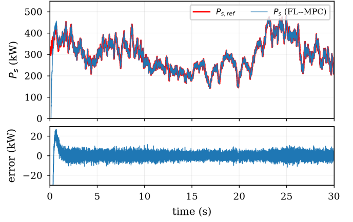
Fig. 6. Active power tracking performance: stator power P_s and MPPT reference P_{s,ref} , and power tracking error.
