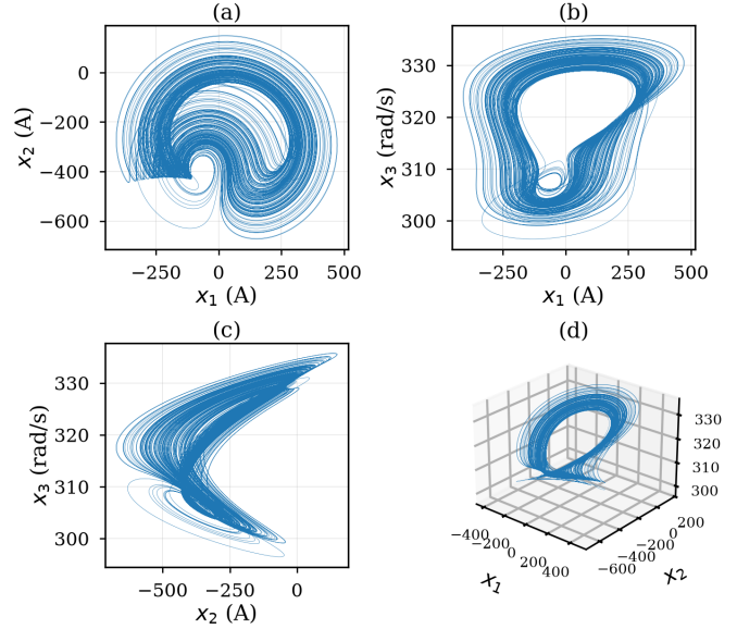
Fig. 1. The chaotic attractors: a) The projection of the chaotic attractor in plan x_1 - x_2 ; b) the projection of the chaotic attractor in plan x_1 - x_3 ; c) the projection of the chaotic attractor in plan x_2 - x_3 ; d) 3D trajectory of the system.
