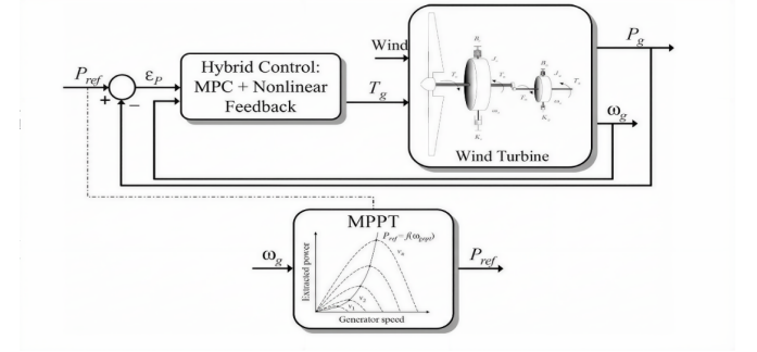
Fig. 3. Proposed hybrid MPC–nonlinear feedback control architecture for DFIG-based wind turbines.
