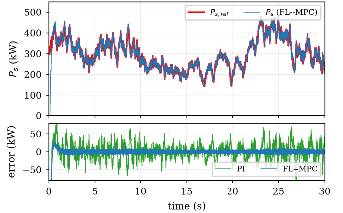
Fig. 6. Active power tracking performance: stator power P_s and MPPT reference P_{s,ref} (FL-MPC), and power errors of FL-MPC and PI.
