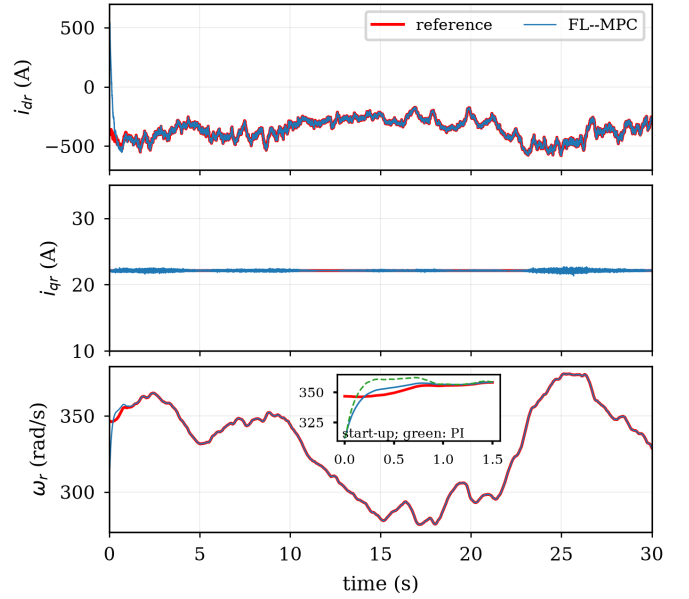
Fig. 5. Tracking performance of the state variables i_{dr} , i_{qr} , and \omega_r under the proposed hybrid control scheme (inset: start-up, green: PI).
