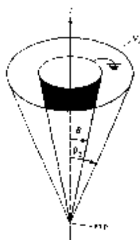
Figure 6.5 Potential V(\theta) due to conducting cones.
