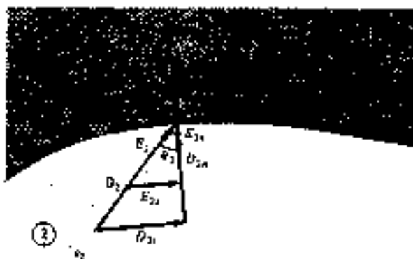
Figure 5.11 Refraction of \mathbf{D} or \mathbf{E} at a dielectric-dielectric boundary
