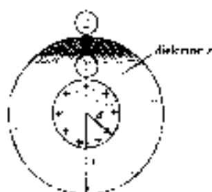
Figure 6.15 Spherical capacitor.
