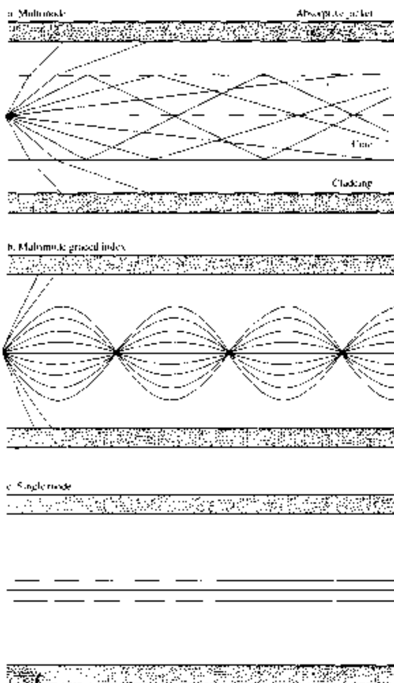
Figure 11.7 Optical fiber transmission modes. (Source: W. Stallings, Local and Metropolitan Area Networks , 4th ed., New York: Macmillan, 1993, p. 95.)
