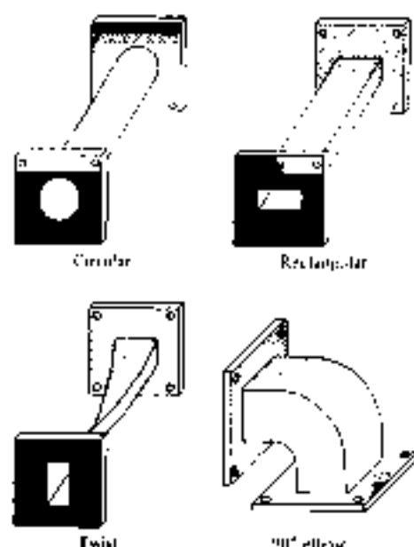
Figure 12.1 Typical waveguides
