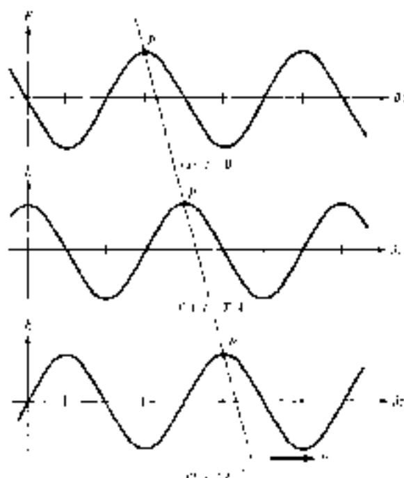
Figure 10.2 Plot of E(z, t) = A \sin(\omega t + \beta z) at time (a) t = 0 , (b) t = T/4 , (c) t = T/2 ; P moves along z direction with velocity v .
