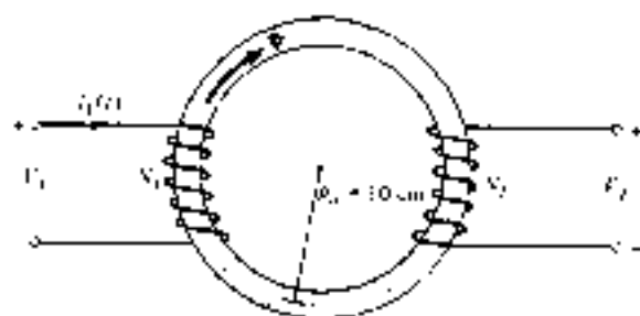
Figure 9.8 Magnetic circuit of Example 9.4.
