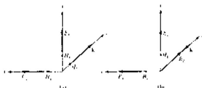
Figure 12.3 Components of LM fields in a rectangular waveguide. (a) TE mode, E_z = 0 , (b) TM mode, H_z = 0 .
