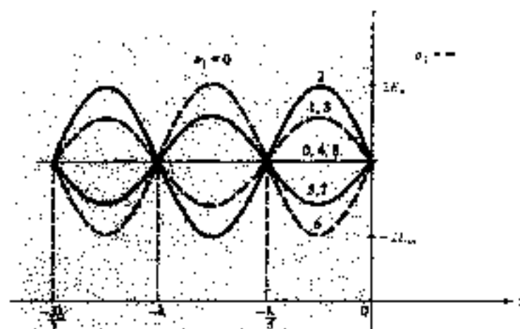
Figure 10.12 Standing waves: E = 2E_0 \sin \beta_1 z \cos \omega t ; curves 0, 1, 2, 3, 4, ... are, respectively, at times t = 0, T/8, T/4, 3T/8, T/2, \dots ; \lambda = 2\pi/\beta_1 .
