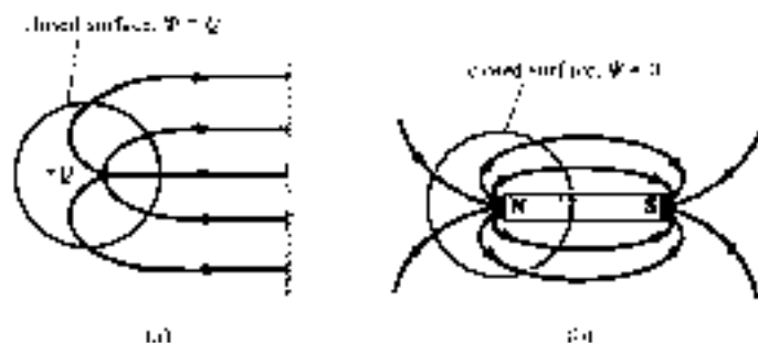
Figure 7.17 Flux leaving a closed surface due to: (a) isolated electric charge \Psi = \oint \mathbf{D} \cdot d\mathbf{S} = Q , (b) magnetic charge \Psi = \oint \mathbf{B} \cdot d\mathbf{S} = 0
