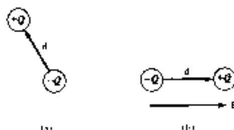
Figure 5.7 Polarization of a polar molecule: (a) permanent dipole ( E = 0 ), (b) alignment of permanent dipole ( E \neq 0 )
