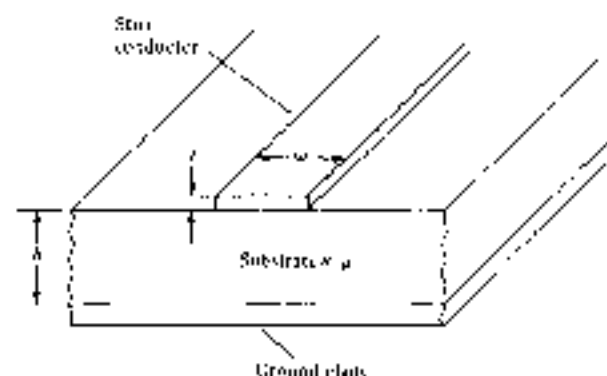
Figure 11.38 Microstrip line.
