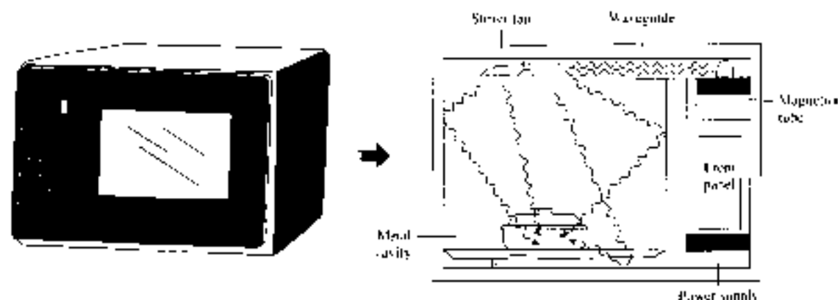
Figure 14.2 Microwave oven. Source: N. Schlager (ed.), How Products are Made , Detroit, MI: Gale Research Inc., 1984, p. 289.
