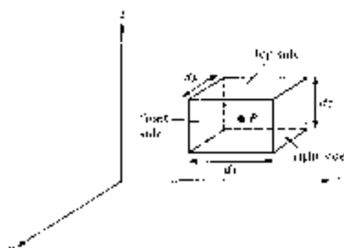
Figure 3.15 Evaluation of \nabla \cdot \mathbf{A} at point P(x, y, z) .
