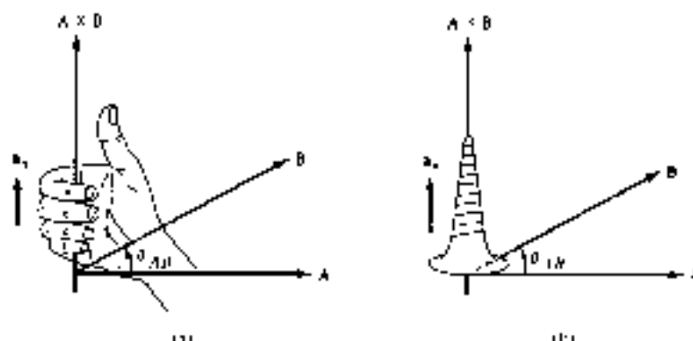
Figure 1.8 Direction of \mathbf{A} \times \mathbf{B} and \mathbf{a}_3 using (a) right-hand rule, (b) right-handed screw rule.
