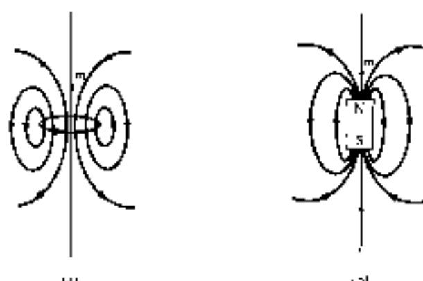
Figure 8.7 The \mathbf{B} lines due to magnetic dipoles: (a) a small current loop with \mathbf{m} = I\mathbf{S} , (b) a bar magnet with \mathbf{m} = Q_m\mathbf{t} .
