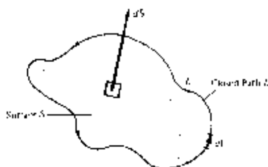
Figure 3.20 Determining the sense of dl and dS involved in Stokes's theorem
