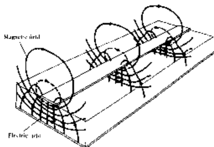
Figure 11.39 Pattern of the EM field of a microstrip line. Source: From D. Rocky, Microwave Technology , 1986, by permission of Prentice-Hall.
