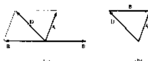
Figure 1.3 Vector subtraction D = A - B : (a) parallelogram rule, (b) head-to-tail rule
