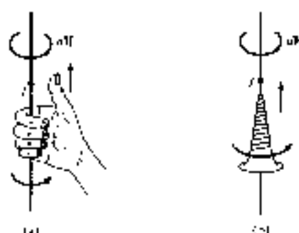
Figure 7.2 Determining the direction of d\mathbf{B} using (a) the right-hand rule, or (b) the right-handed screw rule.
