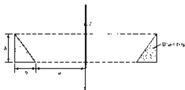
Figure 7.25 Cross section of a brass ring enclosing a long straight wire: for Problem 7.25.
