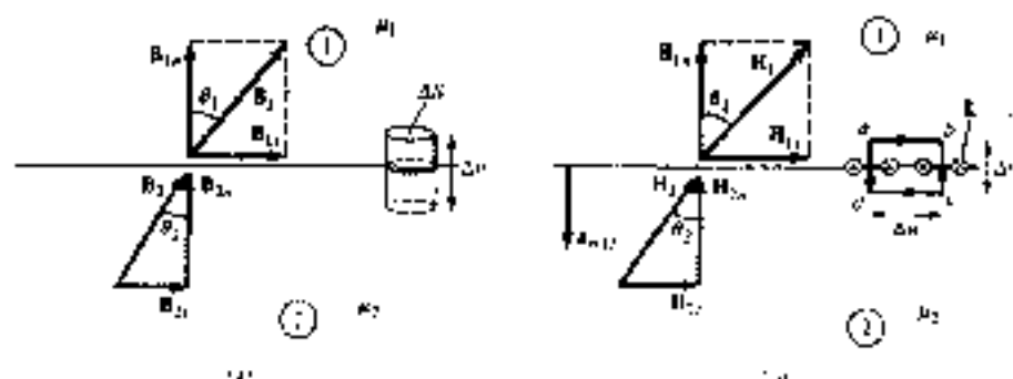
Figure 8.16 Boundary conditions between two magnetic media: (a) for \mathbf{B} , (b) for \mathbf{H} .
