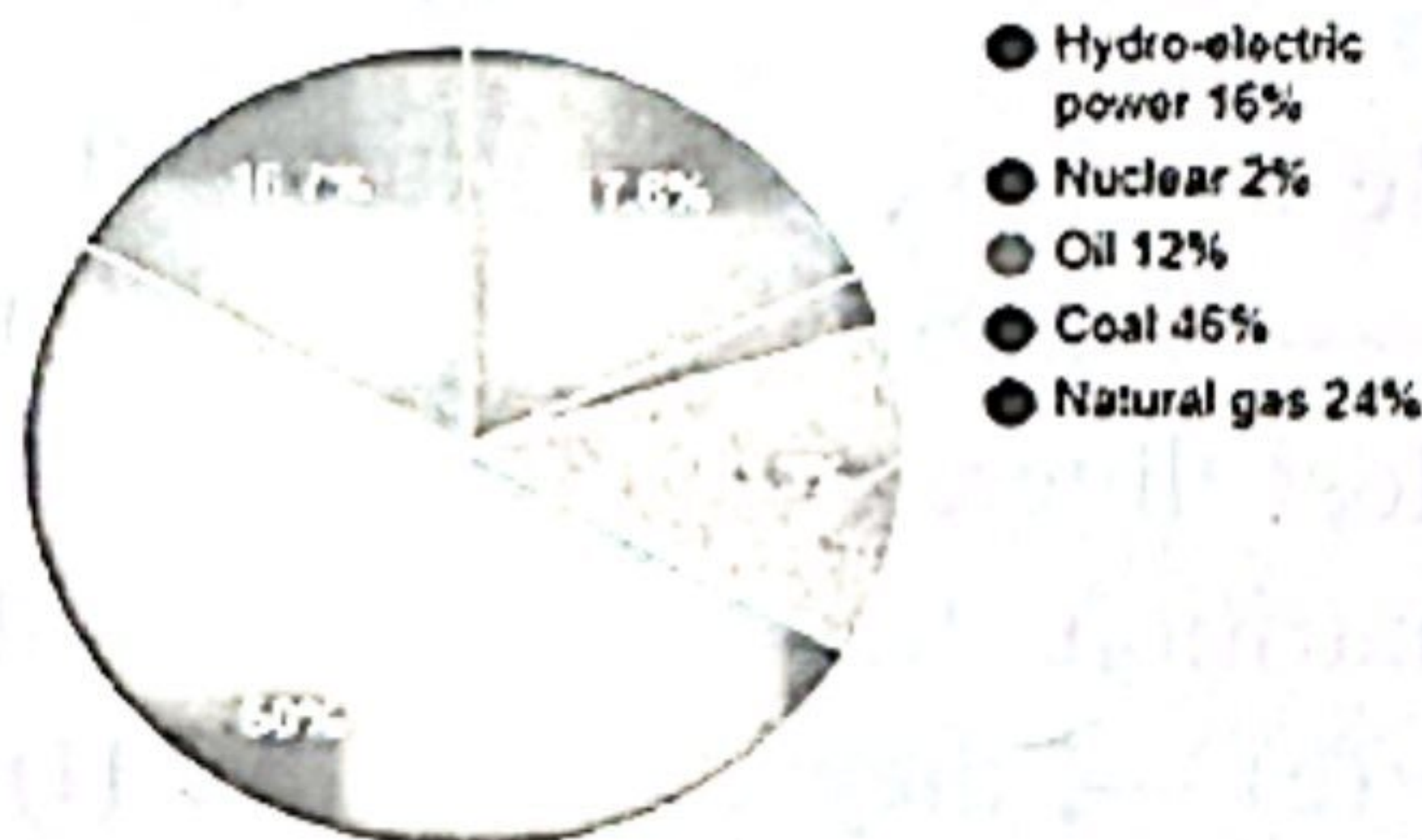
Sources of USA electricity in 1980
