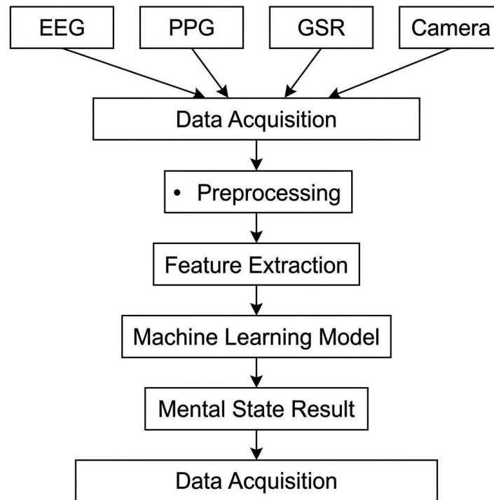
Figure 4.3.3 Software architecture
