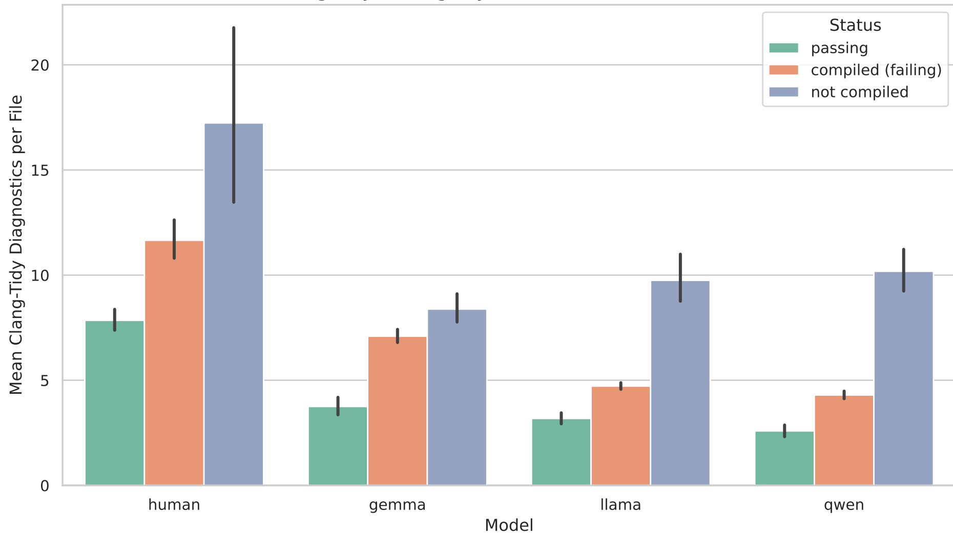
Clang-Tidy Findings by Model and Solution Status
