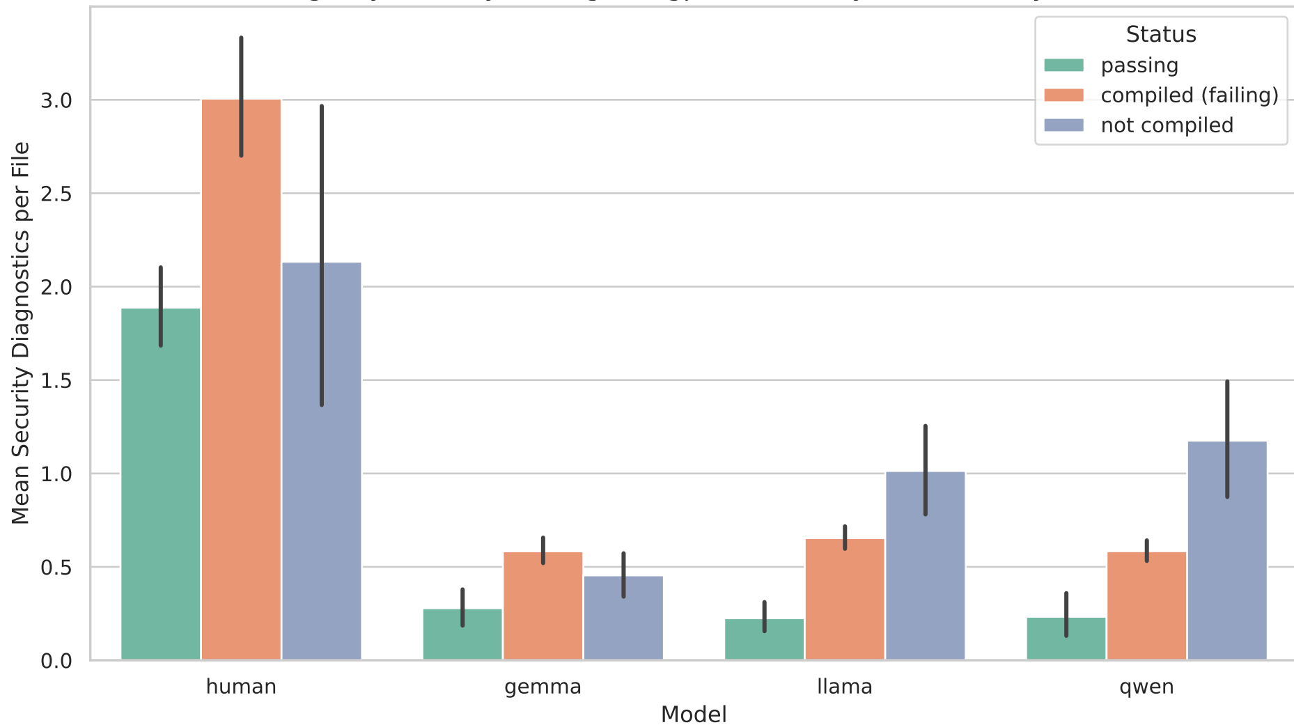
Clang-Tidy Security Findings (bugprone + analyzer + cert) by Status
