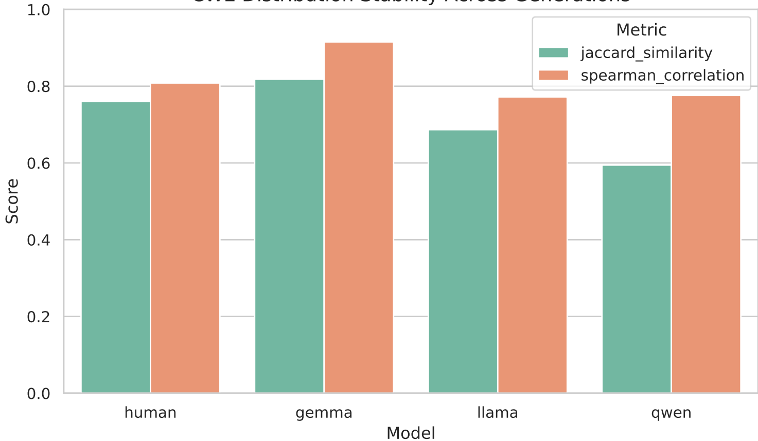
CWE Distribution Stability Across Generations
