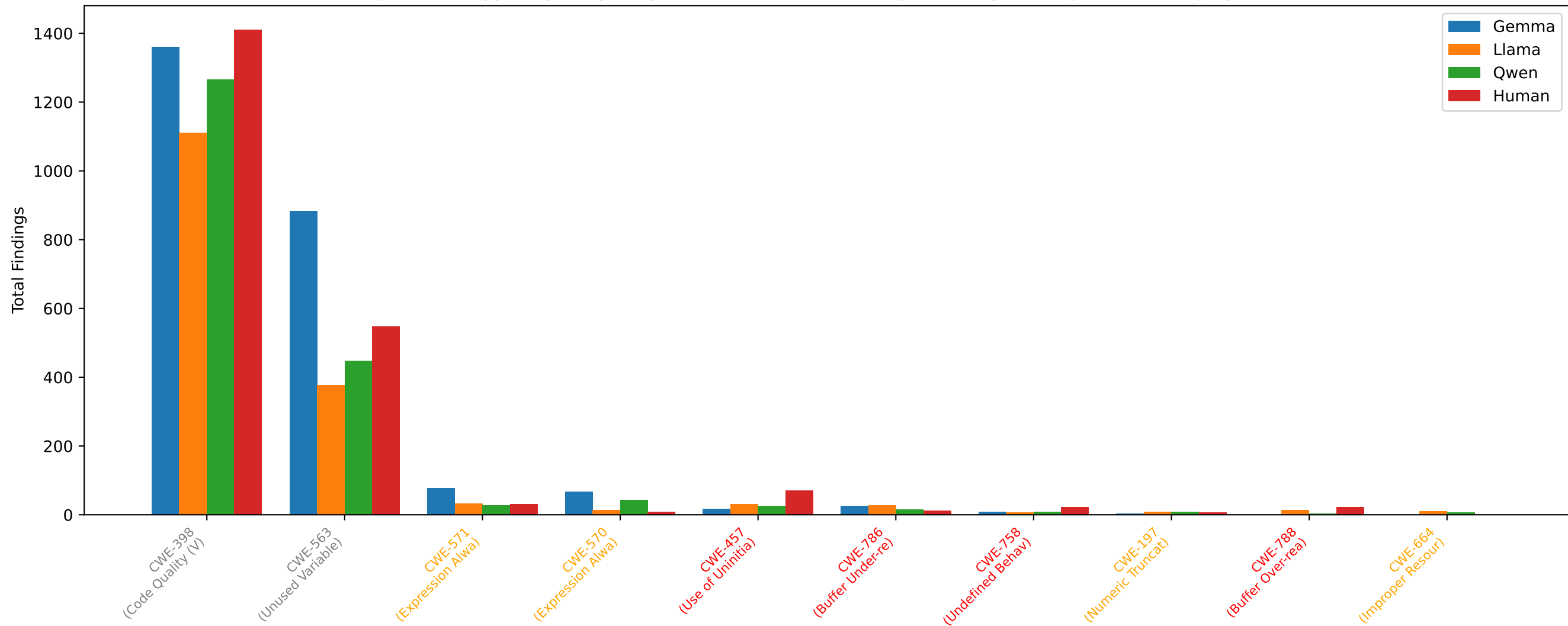
Top 10 CWE Types by Frequency (colored labels = severity: red=High, orange=Medium, gray=Low)
