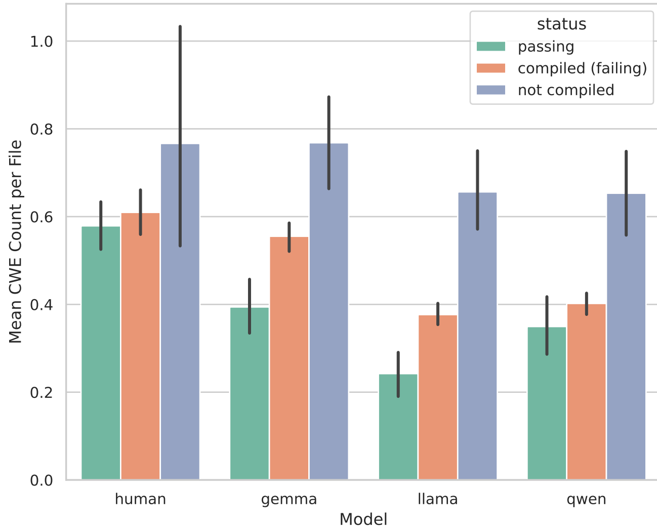
cppcheck CWE per File by Status
