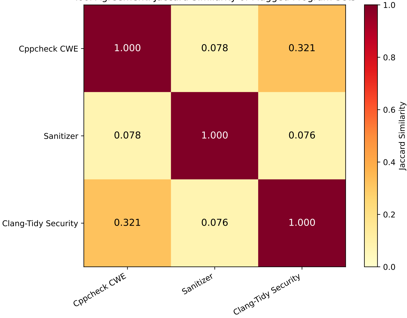
Tool Agreement: Jaccard Similarity of Flagged Program Sets
