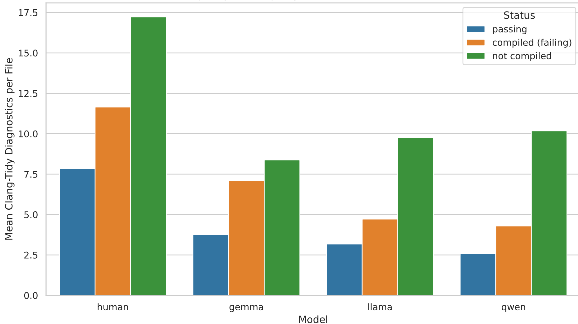
Clang-Tidy Findings by Model and Solution Status
