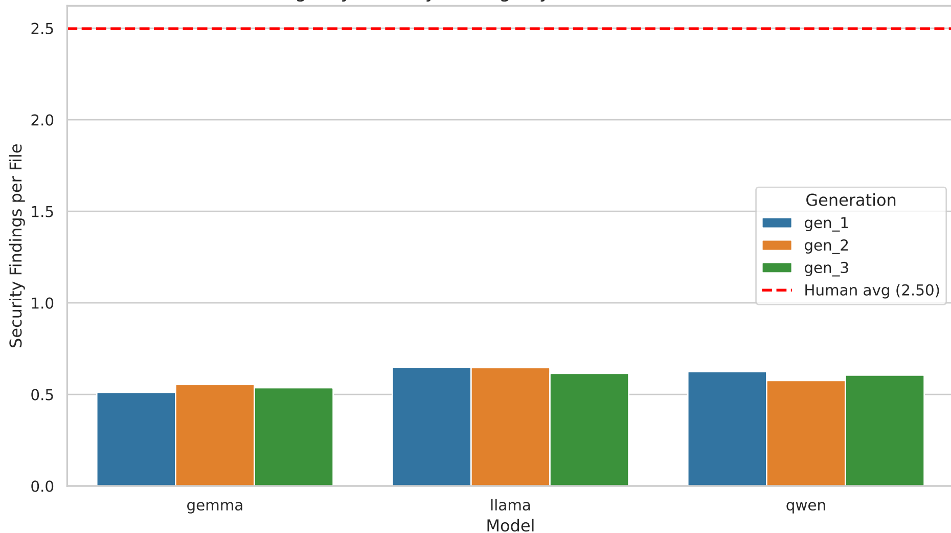
Clang-Tidy Security Findings by Model and Generation
