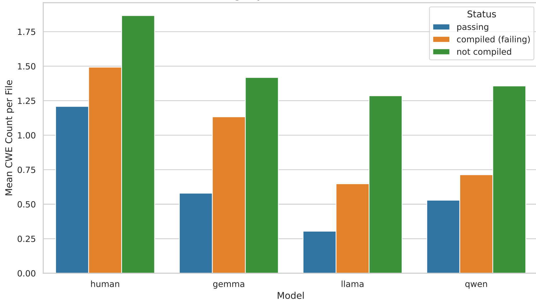
CWE Findings by Model and Solution Status
