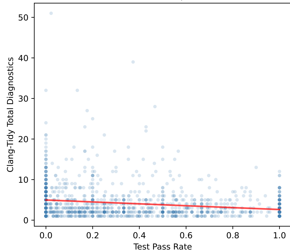
Qwen (rho=-0.248, p=8.33e-21)
