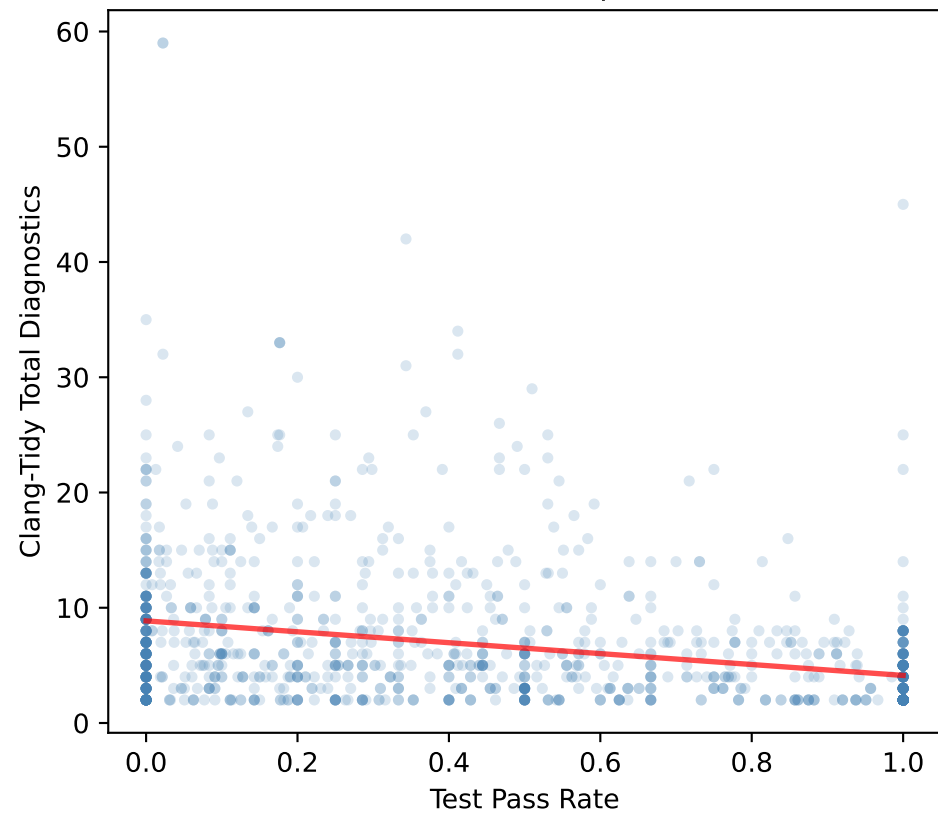
Gemma (rho=-0.368, p=6.84e-40)
