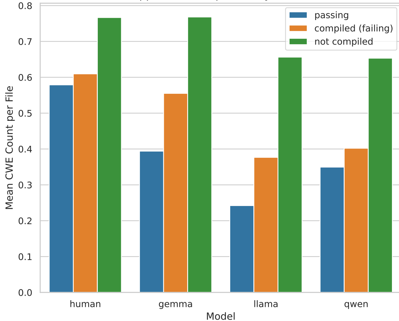
cppcheck CWE per File by Status
