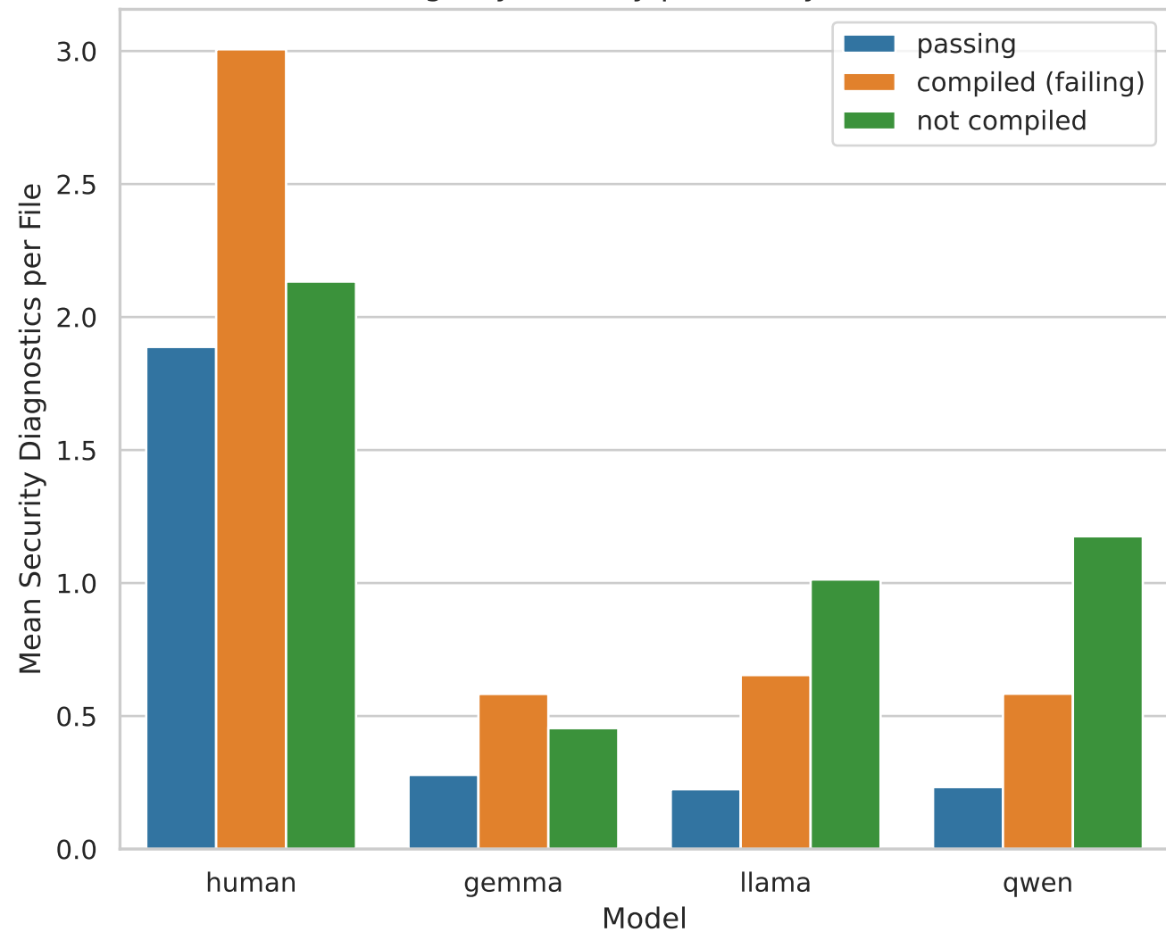
clang-tidy Security per File by Status
