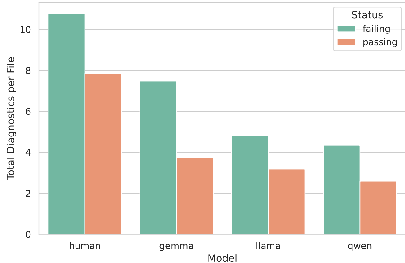
Clang-Tidy Total Diagnostics by Pass/Fail Status
