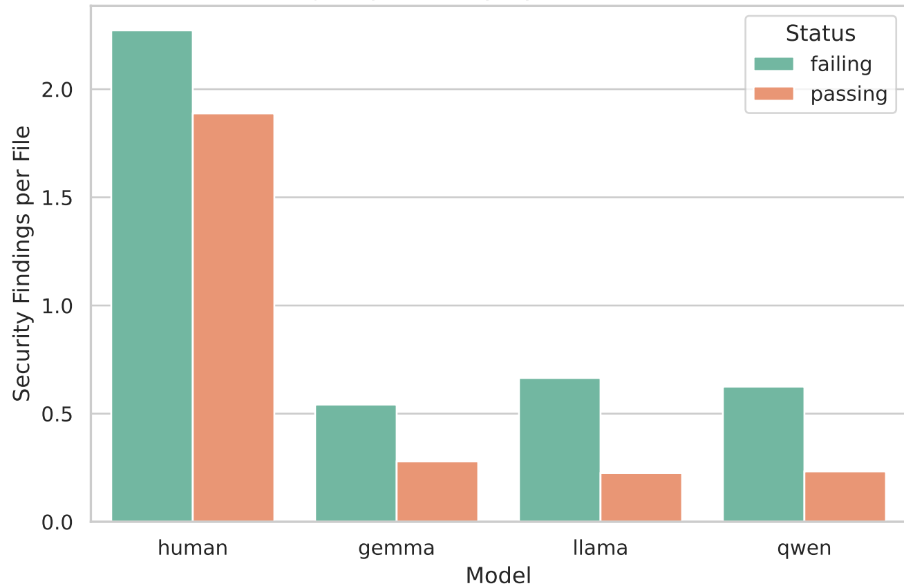
Clang-Tidy Security by Pass/Fail Status
