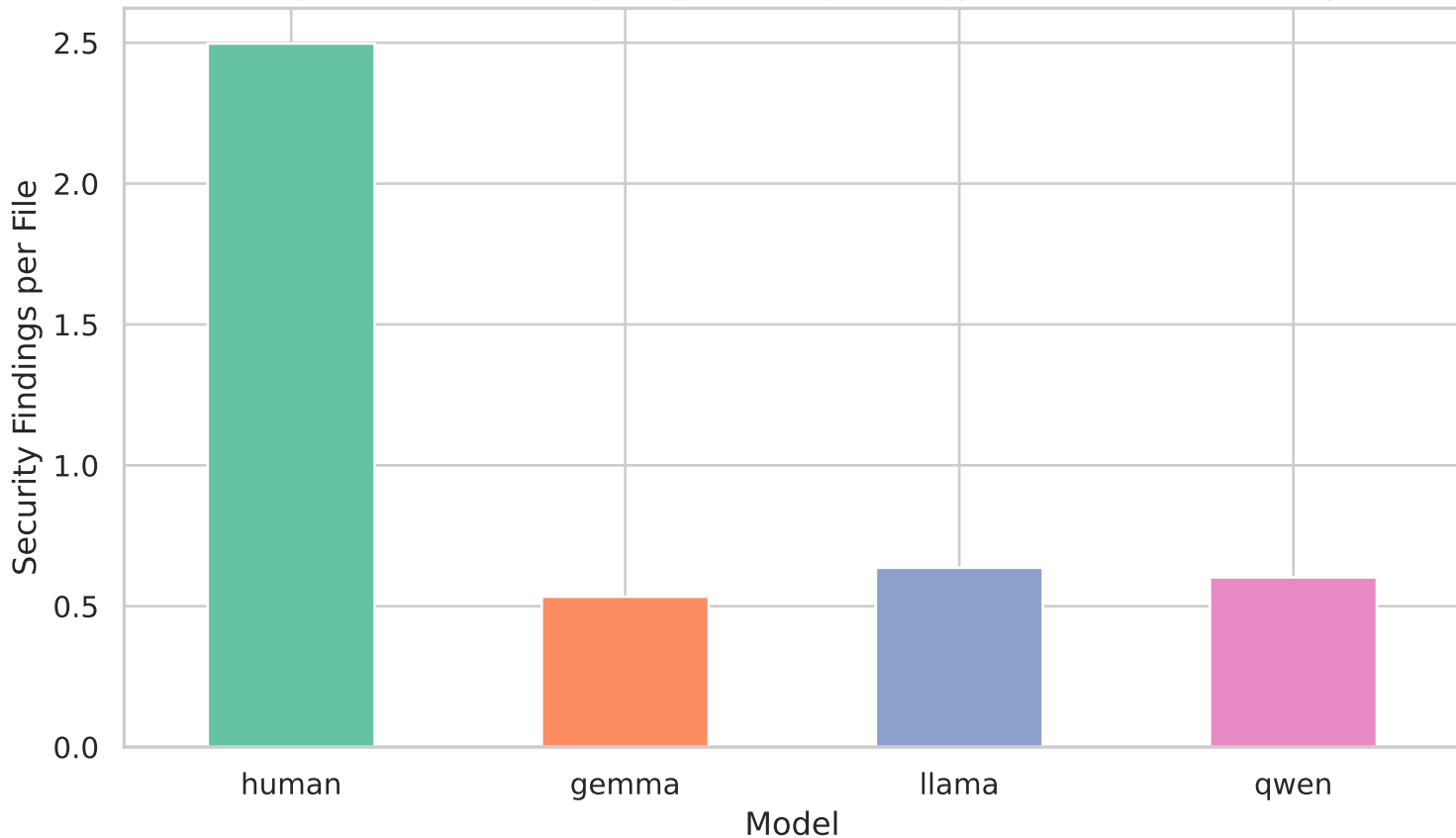
Security-Relevant Clang-Tidy Findings (bugprone + cert + analyzer)
