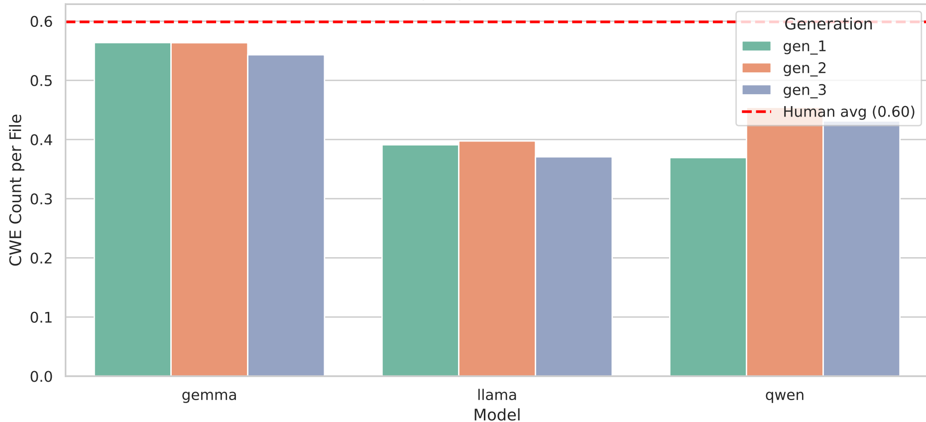
CWE Findings by Model and Generation
