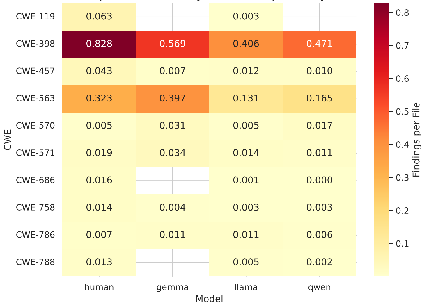
Top 10 CWE Rates by Model (Compiled Only)
