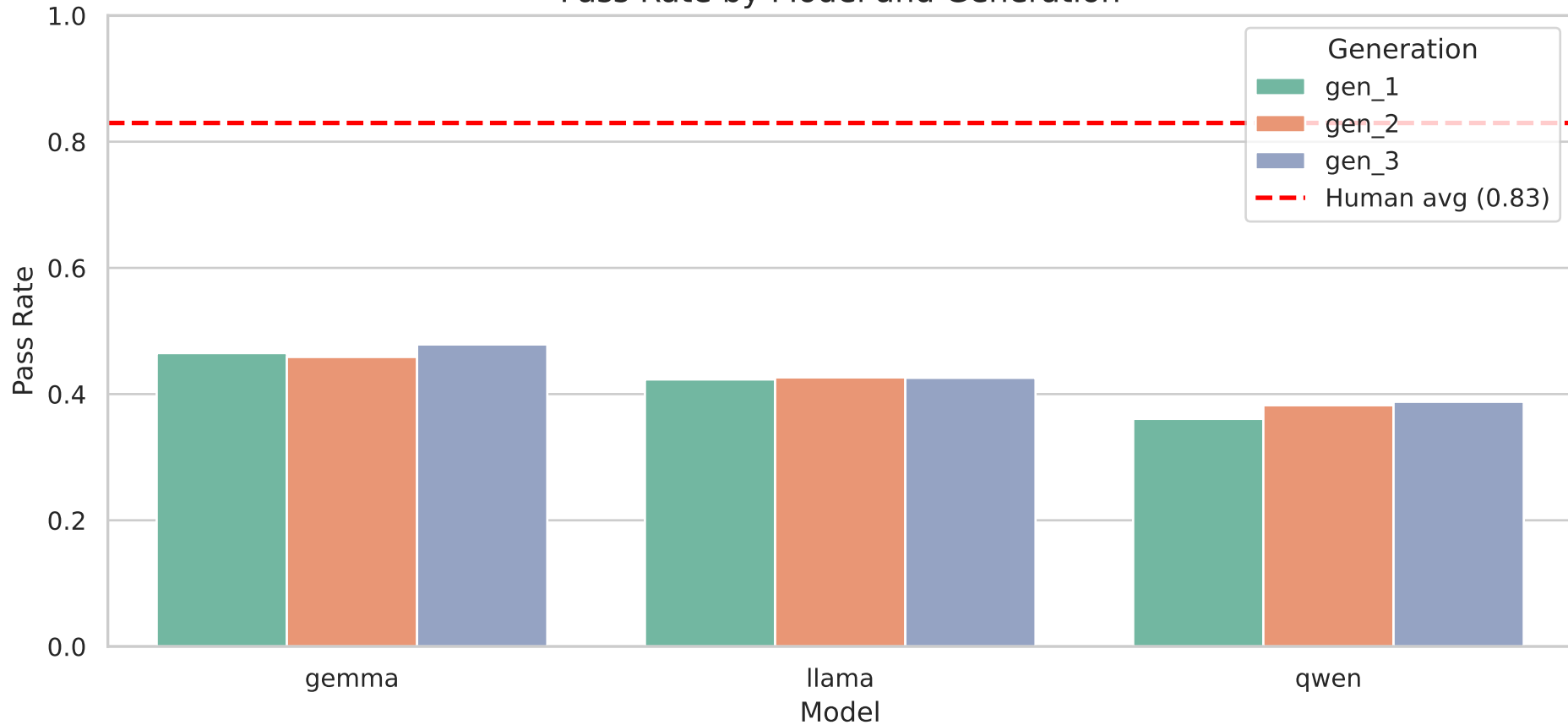
Pass Rate by Model and Generation
