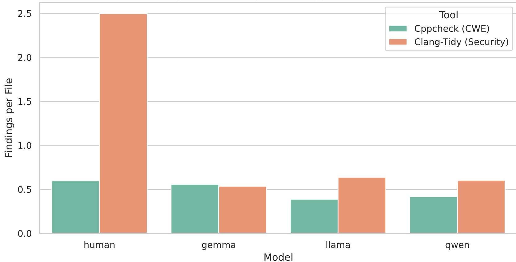
Static Analysis Tool Comparison: Cppcheck vs Clang-Tidy
