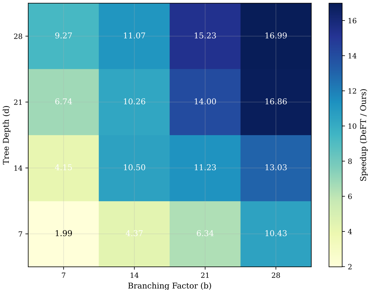
Balanced Tree-Attention Speedup over DeFT: Depth vs Branching Factor (Batch Size=1, Prefix=0)
