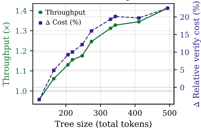
A100 Tree Size Sweep (L=4096)
