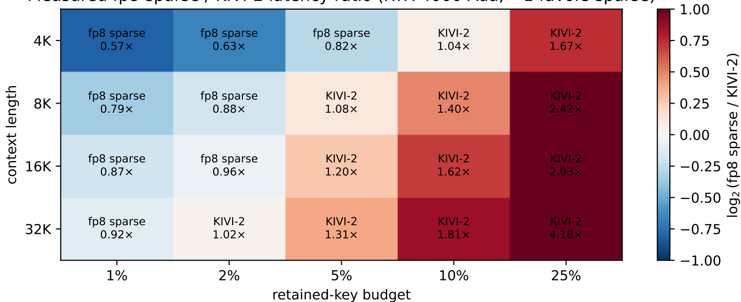
Measured fp8-sparse / KIVI-2 latency ratio (RTX 4000 Ada; <1 favors sparse)
