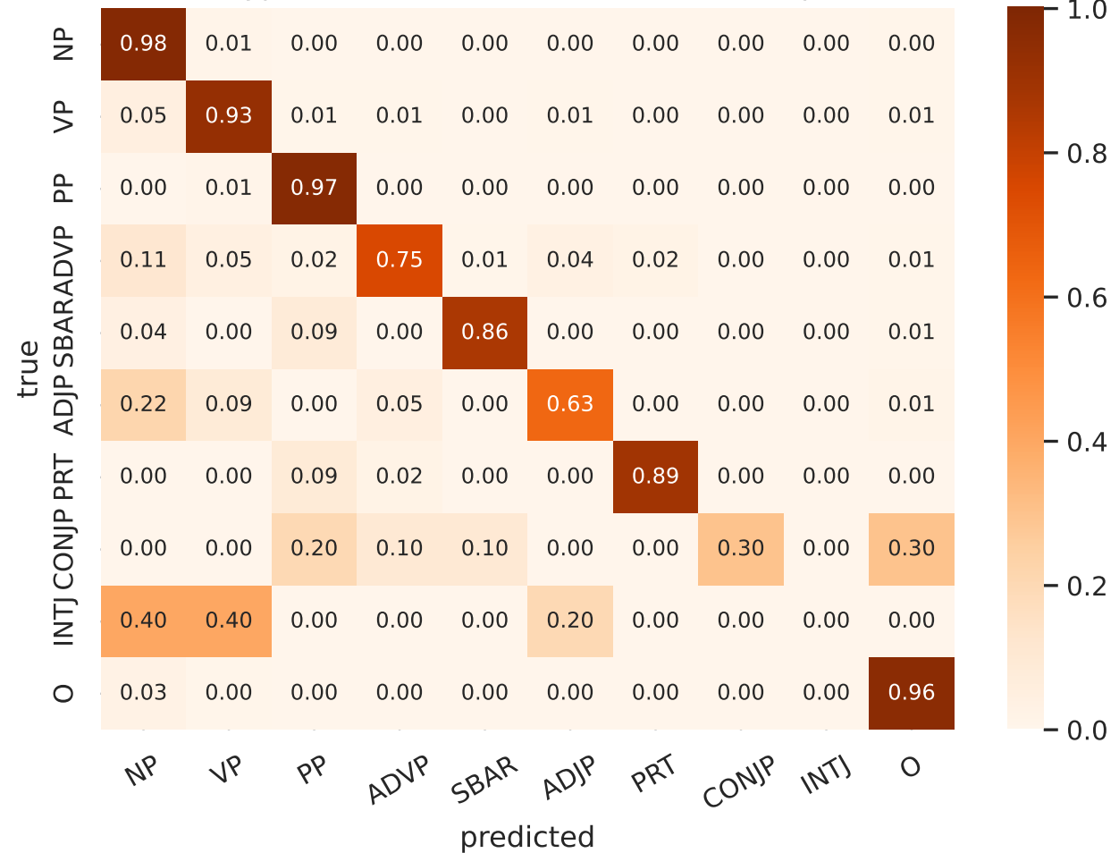
Chunk-type confusion (row-normalised) — DeepBiLSTM
