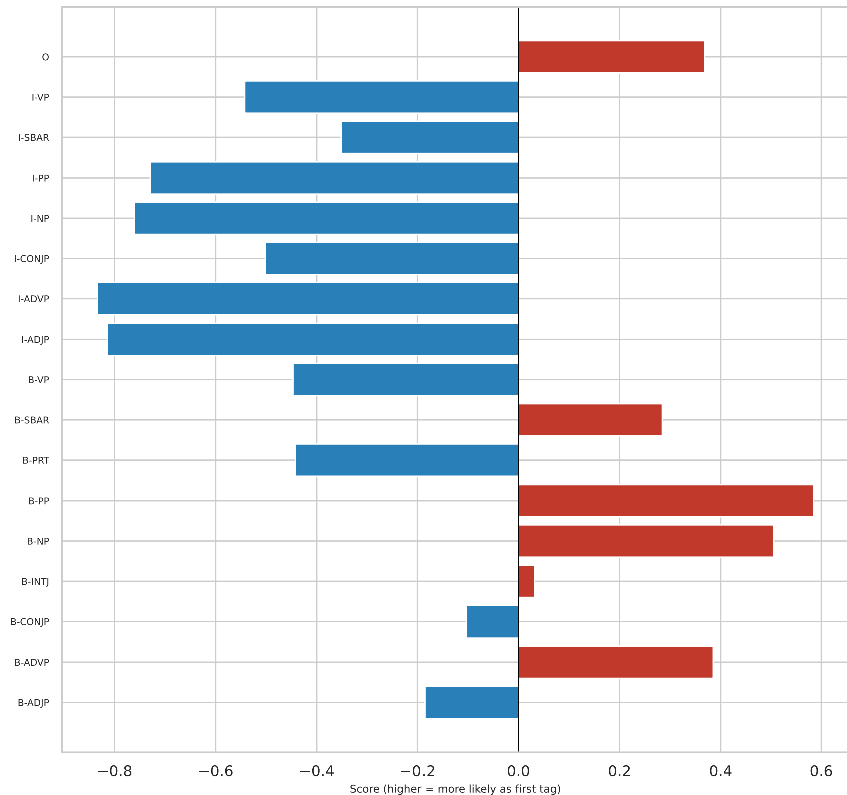
BiLSTM+CRF — start transitions
