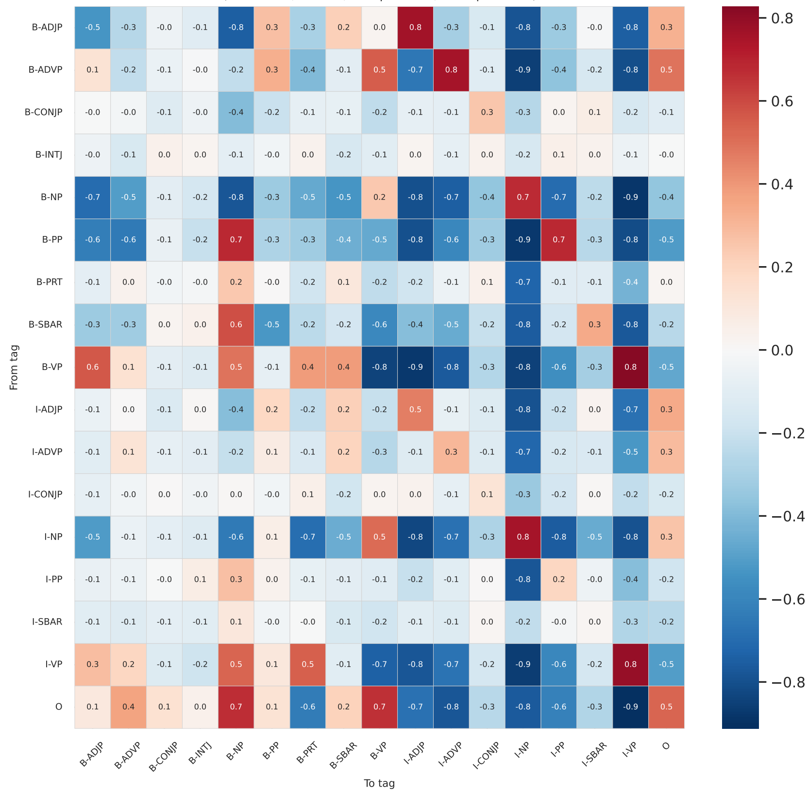
Transformer+CRF — CRF transition matrix
