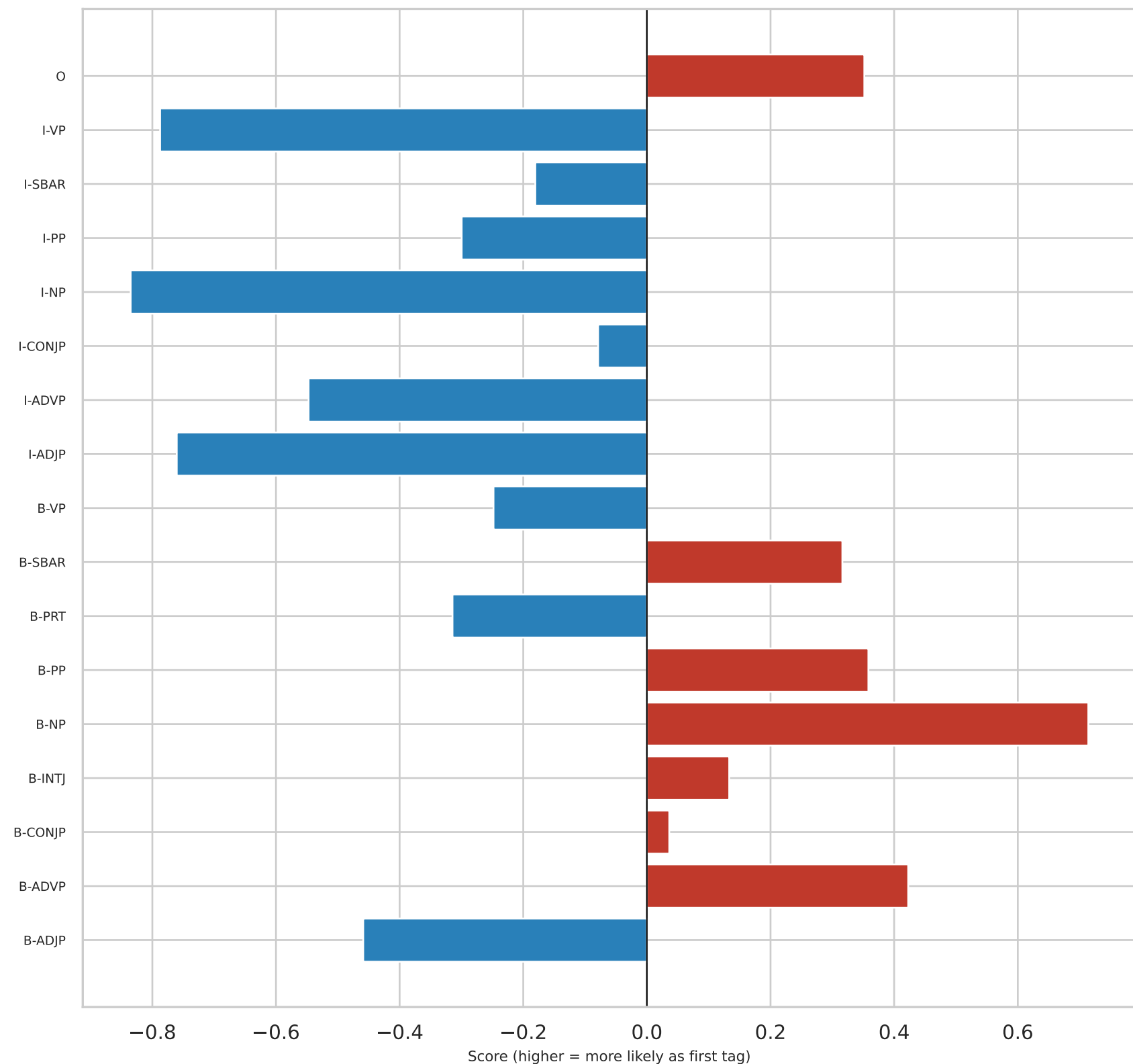
Transformer+CRF — start transitions
