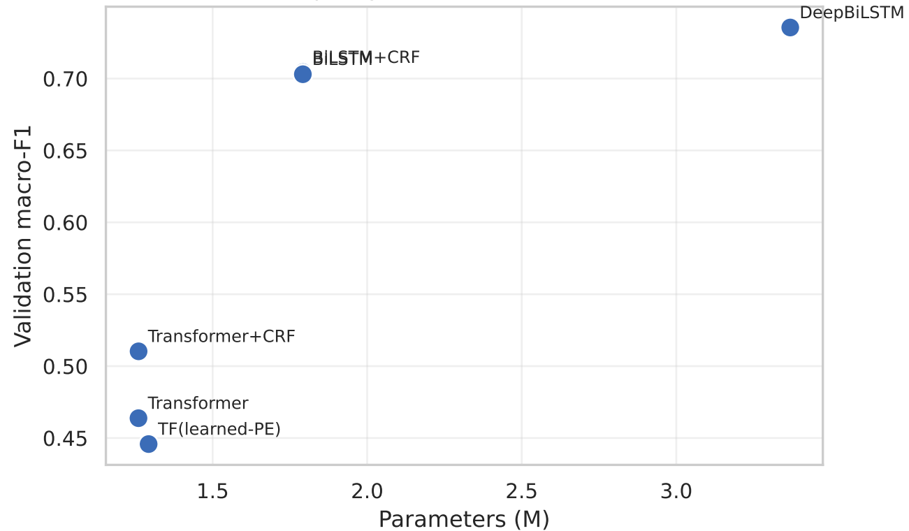
Capacity vs validation macro-F1
